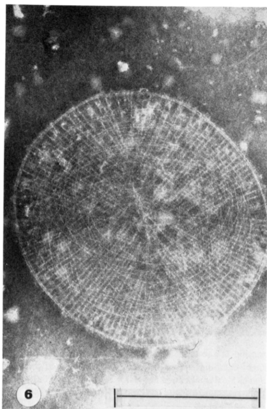
FIG. 6. Negative stain preparation (phosphotungstic acid) of the subtending circular scale. Note the typical quadriradial microfibrillar network, the sparse and poorly organized spiral microfibrillar network, and the rim of doublet microfibrils. Magnification bar = 0.25 \mu\text{m} . ( Cricosphaera ).
