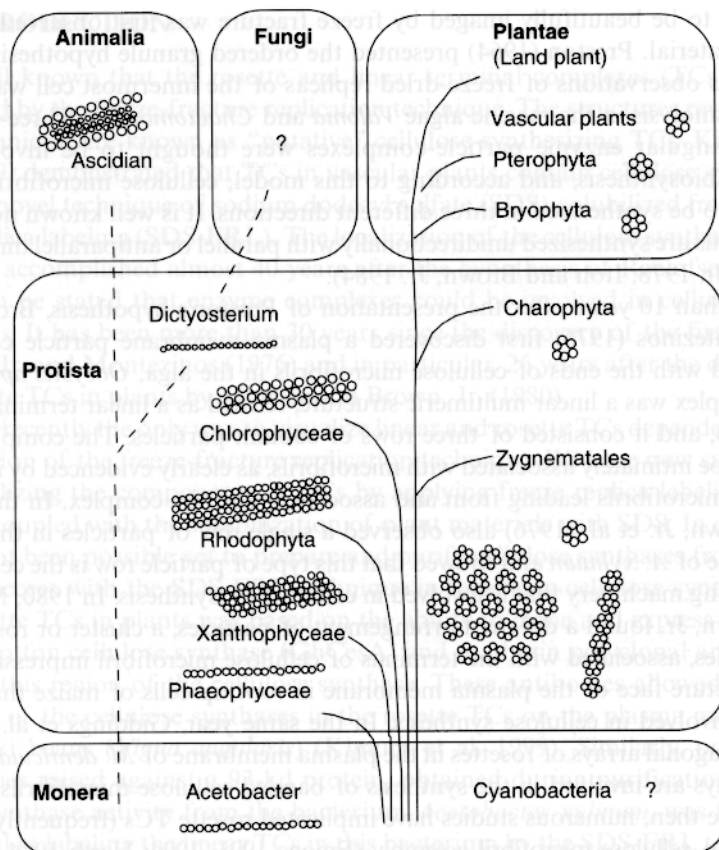
Figure 14-1. Different morphological forms of cellulose-synthesizing terminal complexes in five different biological kingdoms. (Figure 1 from: Itoh, T. 2002. Immunogold labeling of terminal cellulose-synthesizing complexes-demonstration coupled by freeze fracture and immunogold labeling techniques. Regulation of Plant Growth and Development (in Japanese) 37:44–50. Reproduced with kind permission of The Japanese Society for Chemical Regulation of Plants.)
