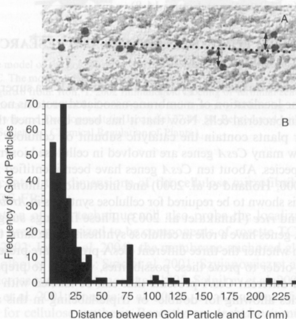
Figure 14-7. The distribution of gold particles associated with linear TCs in A. xylinum . (Figure 4 from: Kimura, S., Chen, H.P., Saxena, I.M., Brown, Jr. R.M., and Itoh, T. 2001. Localization of c-di-GMP-binding protein with the linear terminal complexes of Acetobacter xylinum . J Bacteriol 183:5668–5674. Reproduced with kind permission of the American Society for Microbiology).
